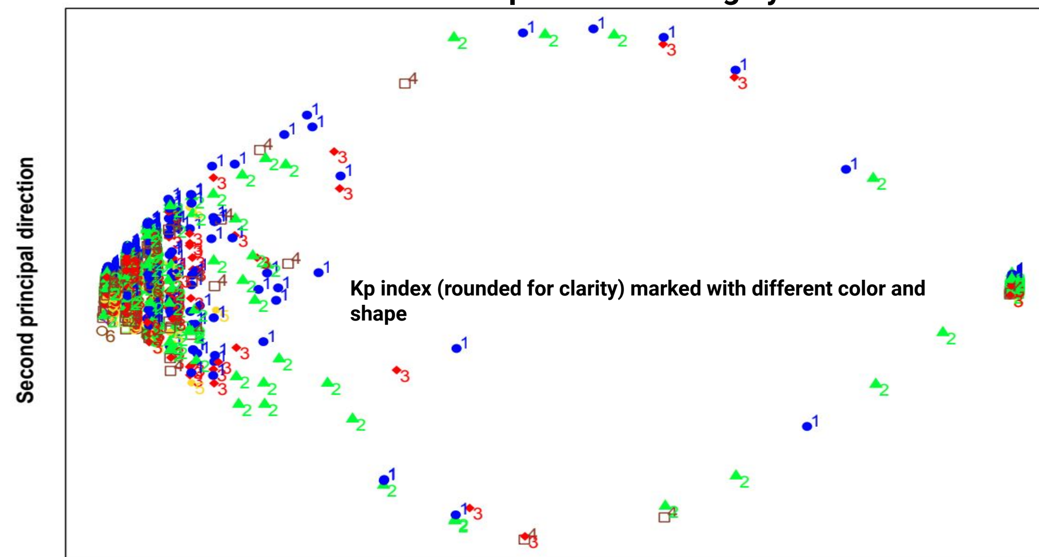
2D visualization of data used in training (originally 100 dimensions). The two dimensions in the graph are top two principal components (directions that data stretches the most). Figure shows how points with different Kp indices can be close, or similar feature conditions can lead to very different Kp indices. It also shows the highly nonlinear pattern between Kp indices and solar activity data.
